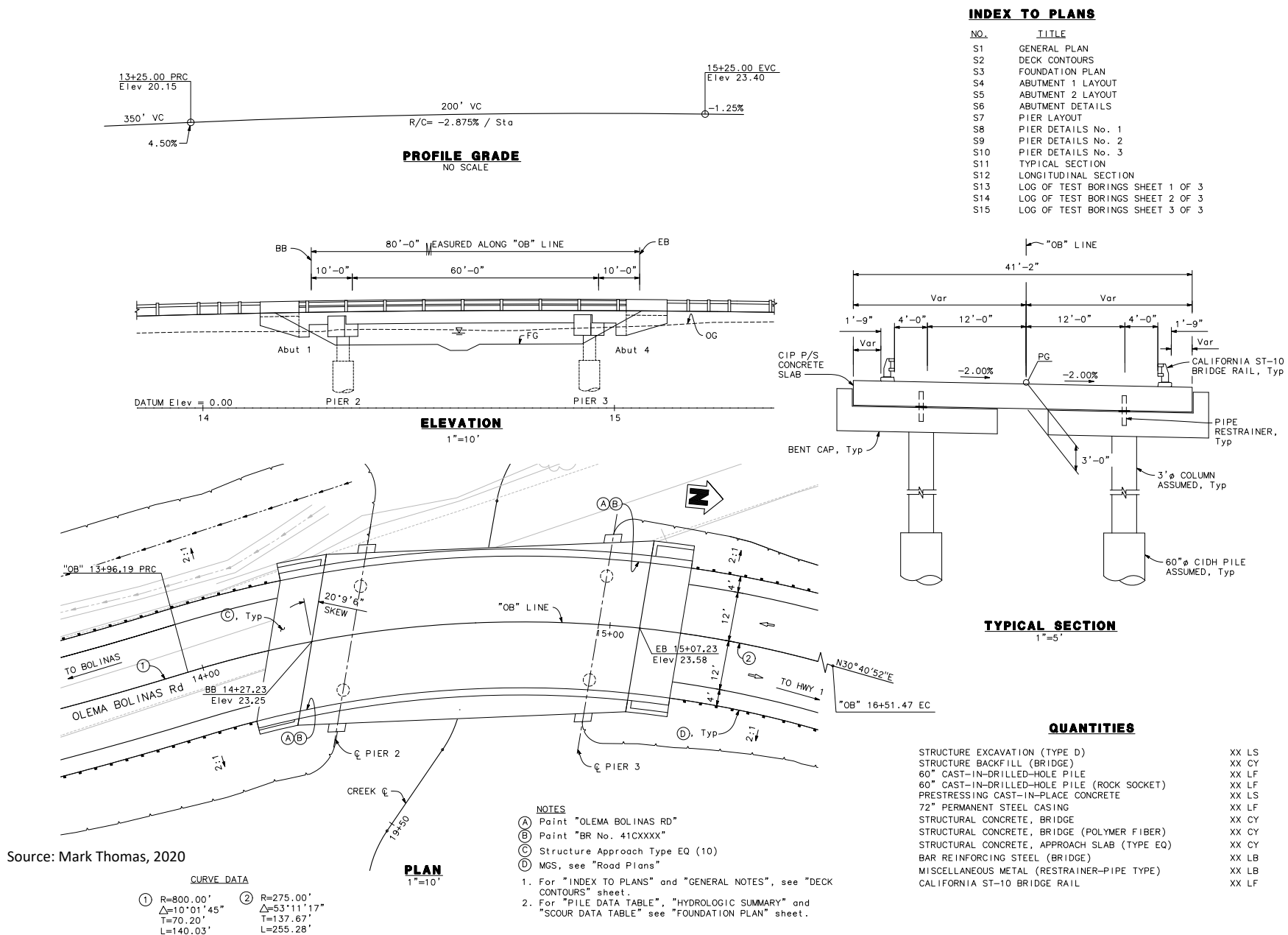
Figure 9. Proposed Bridge Design
