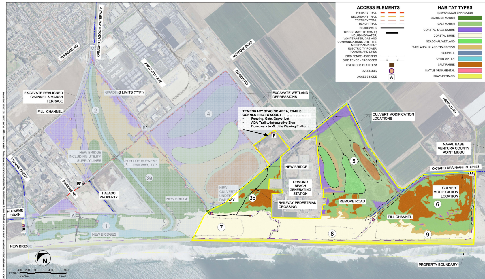
Figure ES-3 Preferred Alternative and Preliminary Design of the Ormond Beach Restoration and Public Access Project First Phase
