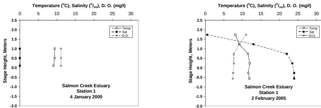
Figure 3.3.3 Bar open water quality profiles. Storm flows sufficient to flush out saltwater are shown on the left and saltwater intrusion after normal base flows return is shown on the right.
