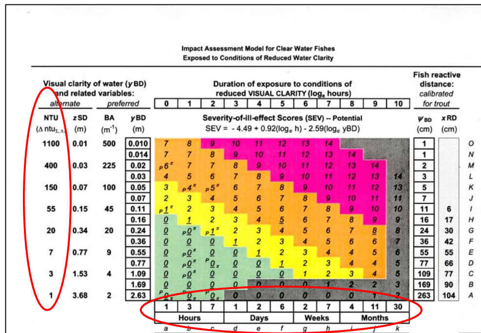
Figure 3.2.6 Newcombe's (2001) turbidity impact model. Severity of impact to salmonids and other clear water fishes increases with NTU (y axis) and time (x axis). Green indicates ideal conditions, yellow slightly impaired, orange significantly impaired, and red is severely impaired. Increasing severity leads to reduced growth and habitat, and/or physiologic impairment.
