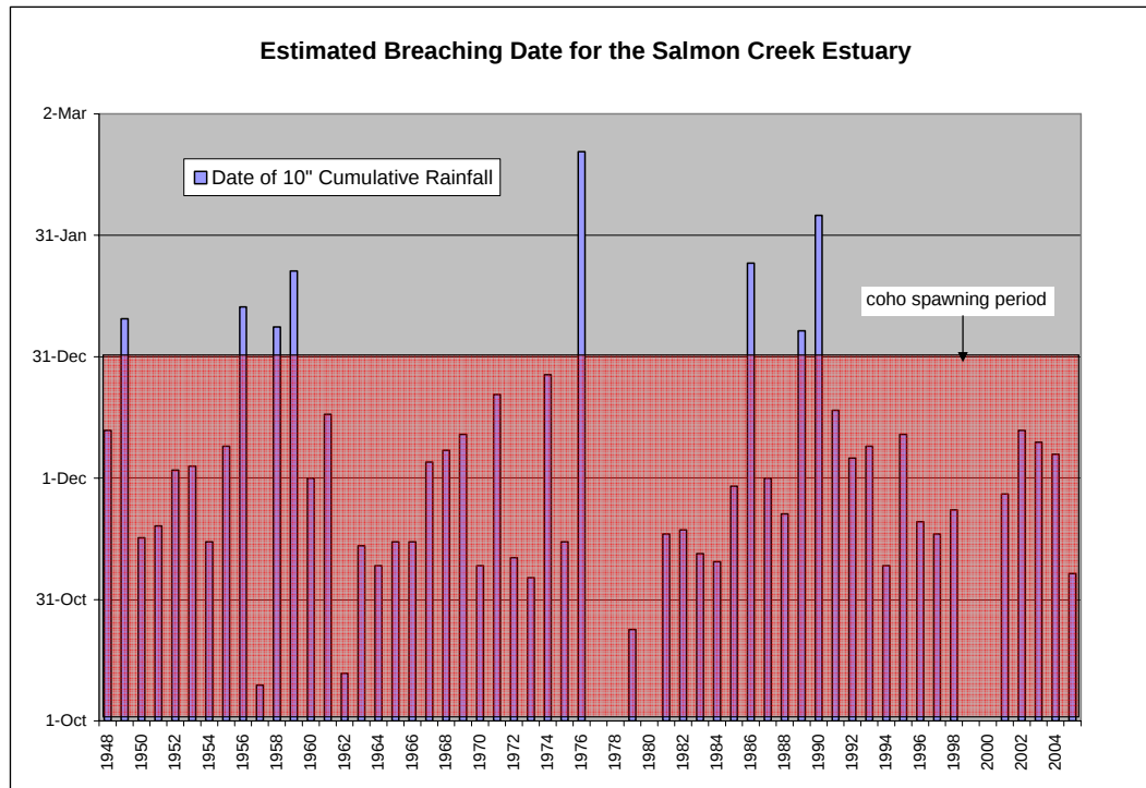
Figure 3.1.9 Dates of initial sandbar opening each fall from 1948 through 2005. It does not appear that the average timing or variation in estuary breaching has changed significantly in the last 60 years. In half of the years there is at least a one month window for coho to enter the watershed for spawning. Occasionally the bar does not open during the coho run period.
