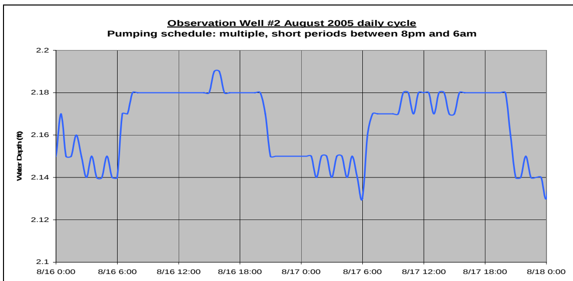
Figure 3.2.4 Examples of daily water table fluctuations in 2004 and 2005. Pattern differences are related to changes in water supply well pumping routines between the two years. Note that in the drought year (2004) the fluctuations were over 2 tenths of a foot, while in the wet year (2005) the fluctuations were only over 6 hundredths of a foot.
