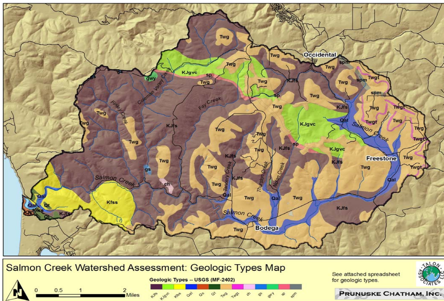
Figure 2.1.2 Watershed geology.
