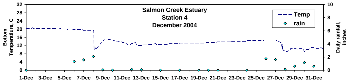
Figure 3.3.6 Temperature response to rainfall events.
