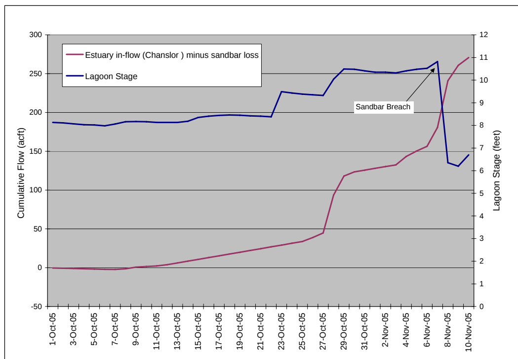
Figure 3.1.7 Lagoon water surface elevations pre- and post-breach 2005 as they relate to stream flows. The sandbar breached on November 8 th . Cumulative inflows were calculated to be approximately 180 acre feet at the time of breach. Given the level of approximation in these estimates, this correlates well with the volume of 135 ac ft needed to fill the lagoon.
