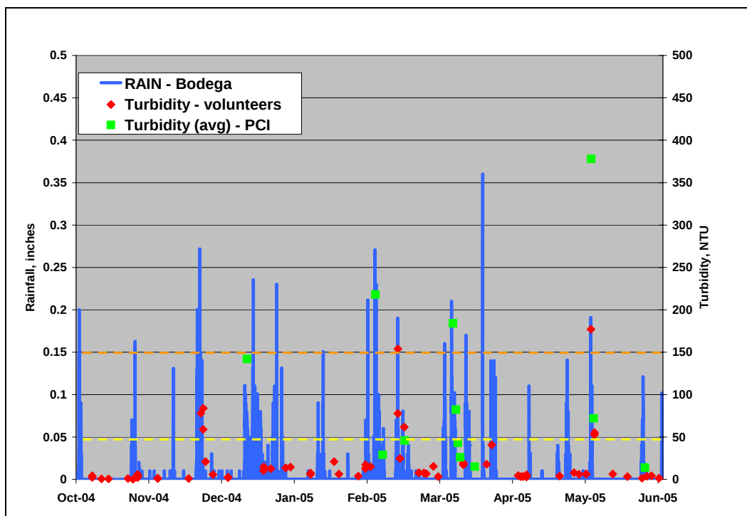
Figure 3.2.5 Turbidity in relation to rainfall in the Salmon Creek watershed. Slight impairment of salmonids occurs under turbidity conditions above the yellow line and significant impairment occurs above the orange line (see Figure 3.2.6)
