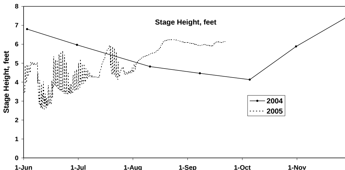
Figure 3.3.8 Comparison of summer stage heights between 2004 and 2005.
