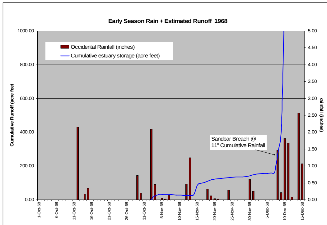
Figure 3.1.8 Example of rainfall/runoff graph used to determine the cumulative rainfall preceding lagoon breaching. As illustrated in this example, runoff during the first rainfalls of the season is minimal, as the majority of the water infiltrates the soil. When the ground reaches saturation, streamflows respond and the flow volumes entering the estuary increase exponentially. Thus, any significant rainfall after the watershed is saturated will likely initiate breaching, regardless of variation in estuary size or antecedent lagoon conditions.
