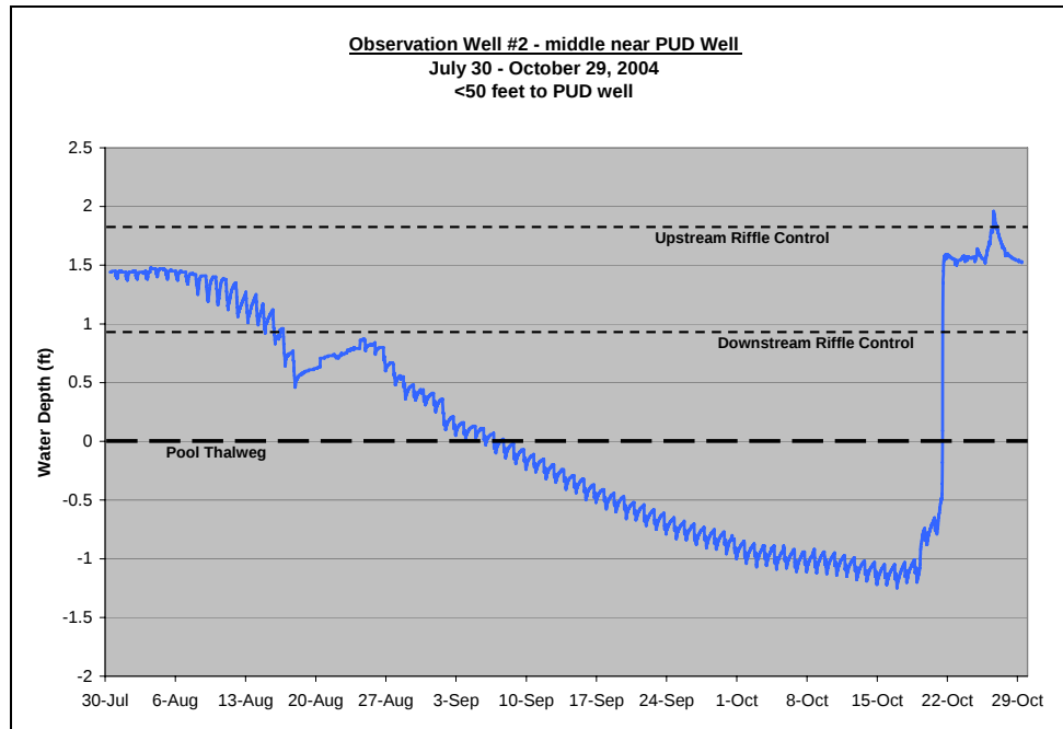
Figure 3.2.2 Water table levels upstream of the estuary in late summer 2004. Timing of pool disconnection and drying is shown when the water levels go below the feature elevations, as well as water table response to the first rain of the season. Daily fluctuations appear to be responses to periods of well pumping.
