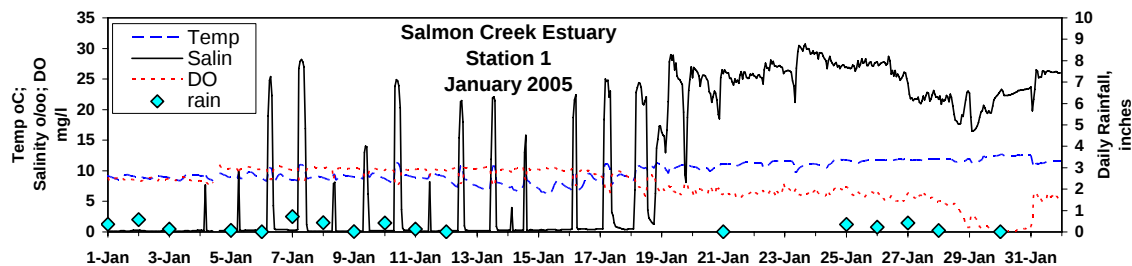
Figure 3.3.4 Records show the influence of tidal and freshwater (rainfall) influx as the estuary mouth is breached.
