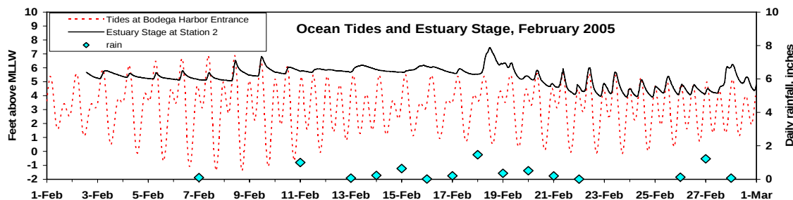
Figure 3.3.7 Ocean tides, estuary stage, and rainfall
