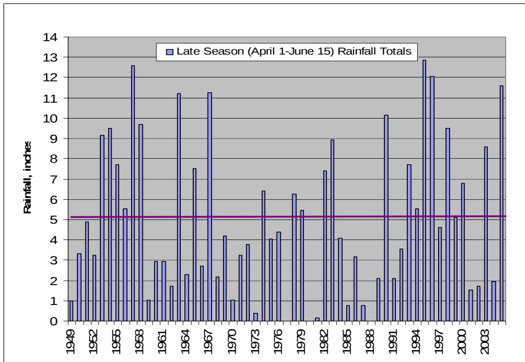
Figure 3.1.6 Spring rainfall totals for the period of record. Higher rainfall during this part of the year translates to longer bar-open conditions in the estuary, higher lagoon elevations in the fall, and sustained summer streamflows in the upper watershed. Conversely, low rainfall during the spring means exacerbated summer drought conditions and poor in-stream and estuarine habitat.
