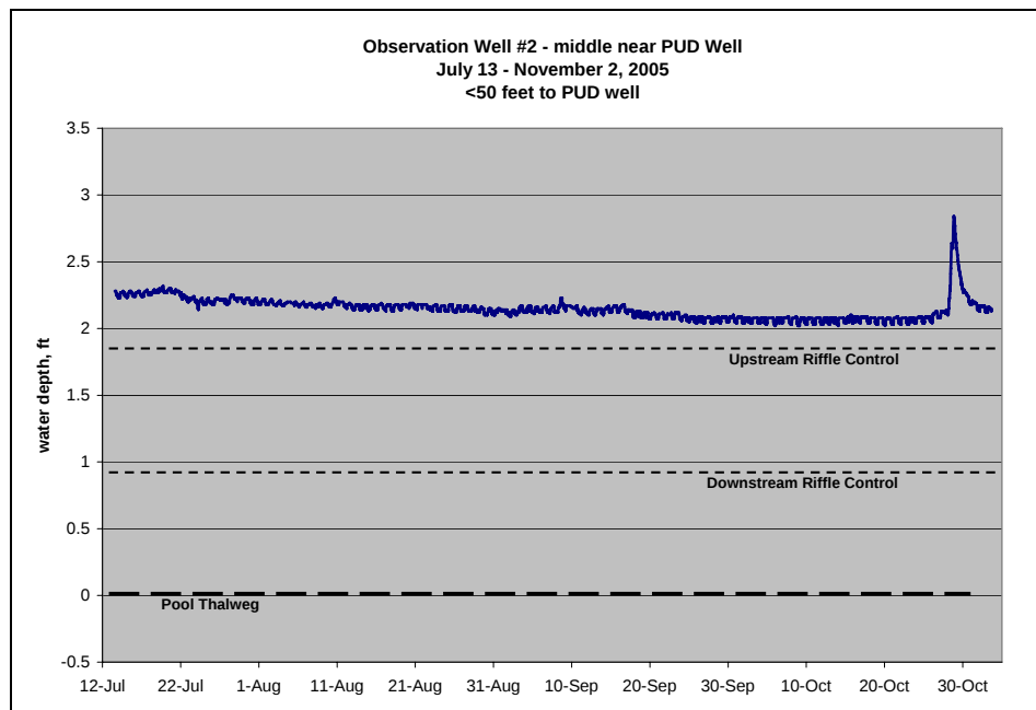
Figure 3.2.3 Water table levels in summer 2005. A wet spring kept the stream and shallow groundwater levels high and consistent through the season. Flows remained well above pool and riffle elevations. Daily pumping of the wells is detectable in the daily fluctuations.
