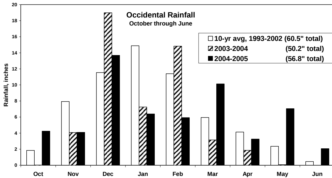
Figure 3.3.9 October through June monthly rainfall summary, 2003-2004 and 2004-2005 seasons compared with the average rainfall for the 10 previous years.
