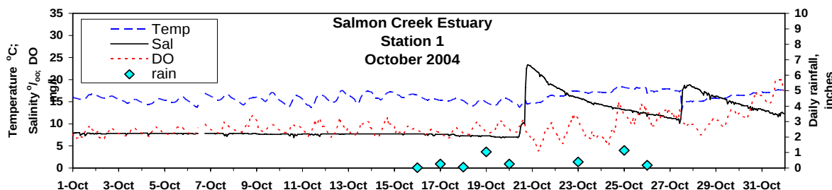
Figure 3.3.2 October, 2004 records show two peaks of saline water entering the lower estuary from upstream. These peaks followed rain events; the beach berm has not been breached to allow tidal waters to enter the estuary.
